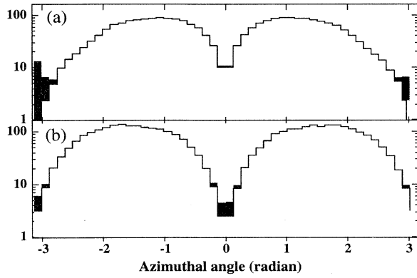
FIG. 3. (a) Azimuthal angular distribution of deflected electrons and positrons ( E_{e\pm} > 100 MeV, \theta_{e\pm} > 0.02 ) for JLC-I. The shaded area corresponds to those positrons that are oppositely charged particles as that of the oncoming beam. (b) The same as (a) except for a zero horizontal crossing angle, i.e., for a head-on collision. The vertical scale is the number of particles per single-bunch crossing.
