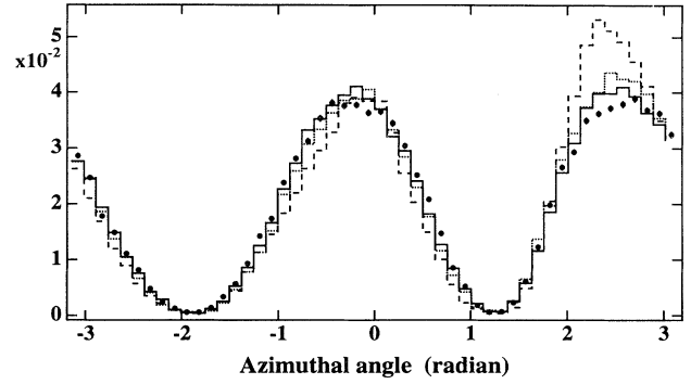
FIG. 10. Azimuthal angular distributions measured for 6 < r < 7 cm at z = +1 m for various transverse rotations compared with the nominal one (solid circles). The signs of the rotations in the xy plane are opposite for two beams, i.e., \phi_{xy} = \pm 0.005 (solid line), \pm 0.01 (dotted line), \pm 0.02 (dashed line) radian. The distributions are normalized by the total number of particles.
