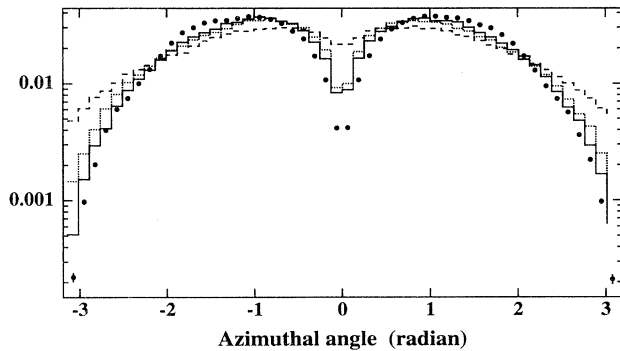
FIG. 4. Azimuthal angular distributions of deflected electrons ( E_e > 100 MeV, \theta_e > 0.02 ), whose charges are the same as that of beam 2 for JLC-I with nominal parameters (solid circles) together with three cases [ \sigma_y = 2\sigma_y^0 (solid line), 3\sigma_y^0 (dotted one), and 10\sigma_y^0 (dashed one)] in which the other beam parameters are the same as those of the nominal beam. The distributions were normalized by the total number of electrons in them.
