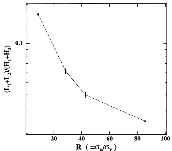
FIG. 8. Number of particles in L_1 and L_2 normalized by that in H_1 and H_2 as a function of R . The same data are used as in the preceding figure. The errors are statistical, corresponding to 160 bunch crossings, except for the lowest R , which corresponds to 800 bunch crossings.
