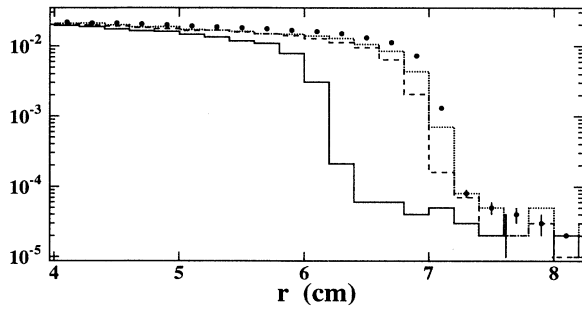
FIG. 6. Radial distribution of scattered particles at z = +1 m. The solid circles are those of the nominal beam condition; the dotted, dashed, and solid lines are those of \sigma_y = 2\sigma_y^0 , \sigma_y = 10\sigma_y^0 , and \sigma_x = 2\sigma_x^0 , respectively, where the other beam parameters are the same as those of the nominal beam. The distributions are normalized by the total number of particles of E > 100 MeV.
