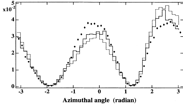
FIG. 9. Azimuthal angular distributions measured for 6 < r < 7 cm at z = +1 m for vertical displacements of \Delta_y = \pm 0.5\sigma_y^0 (solid line), \pm 1.0\sigma_y^0 (dotted line) compared with the nominal one (solid circles). The distributions are normalized by the total number of particles.
