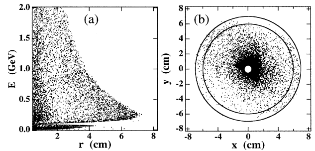
FIG. 5. Distributions of scattered particles at z = +1 m, where particles with r > 0.5 cm are plotted. The particles are tracked in helical trajectories in a magnetic field of B_z = 2 T. (a) is for a scatter plot on the plane of the energy ( E ) and the radial distance ( r ), and (b) is for a plot on the plane of x and y , where two concentric circles of 6- and 7-cm radii are also shown just for an eye guide.
