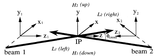
FIG. 2. Coordinate system used in ABEL, where z_1, z_2 , and z are collinear. The trajectories of the beam centers are indicated by the long-thick arrows.
