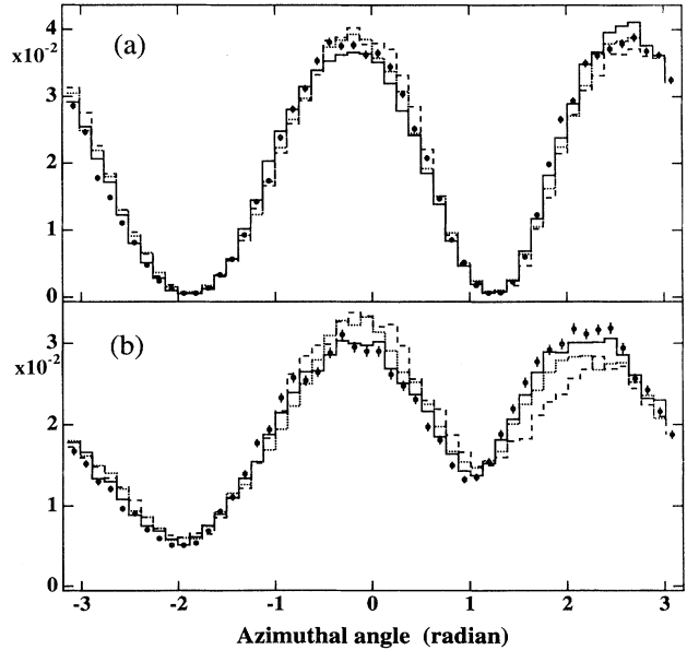
FIG. 11. Azimuthal angular distributions measured for (a) 6 < r < 7 cm and (b) 5 < r < 6 cm at z = +1 m for various rotations compared with the nominal one (solid circles). The magnitudes of the rotations are \phi_{xy} = +0.005 (solid line), +0.01 (dotted line), +0.02 (dashed line) for both beams. The distributions are normalized by the total number of particles.
