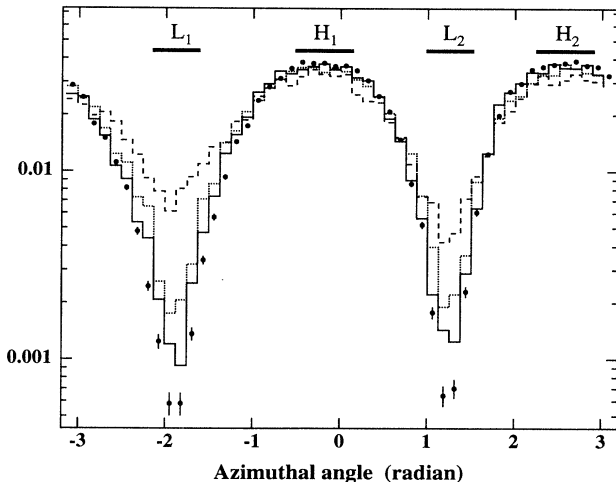
FIG. 7. Azimuthal angular distributions measured for 6 < r < 7 cm at z = +1 m for R = 85.5 (solid circles), 42.8 (solid line), 28.5 (dotted line), and 8.55 (dashed line) corresponding to \sigma_y = \sigma_y^0 , 2\sigma_y^0 , 3\sigma_y^0 , and 10\sigma_y^0 , respectively. The distributions are normalized by the total number of particles. The angular regions of L_1 (left), L_2 (right), H_1 (down), and H_2 (up) are also shown.
