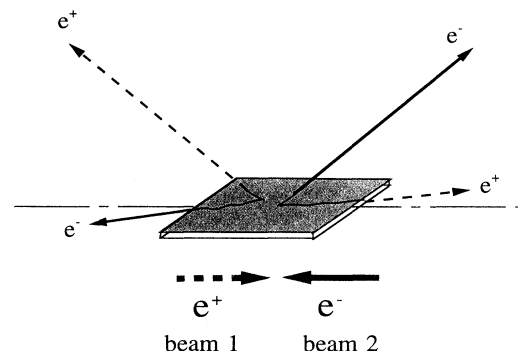
FIG. 1. Schematic view of e^+e^- pair creations and deflections during a collision, where two flat beams are depicted as overlapping sheets at the IP and two e^\pm pairs are created in forward and backward angles, only as an example.
